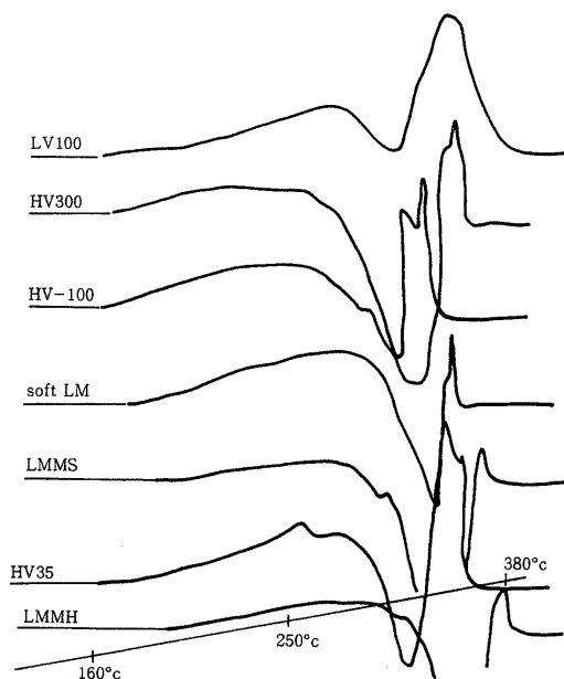
Fig.4 DTA curve of polybutene & polyisobutylene DTA range : 25 \mu v/heating temp rate 5 °C/min chart speed : 2.5 mm/min, standard : \alpha - \text{Al}_2\text{O}_3 thermo couple : Pt - Rh
