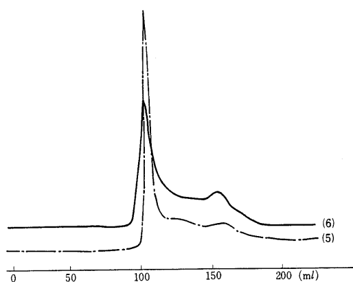
Fig. 14 Gel permeation chromatogram (RI Curve) (5)Sample E (6)Sample F
