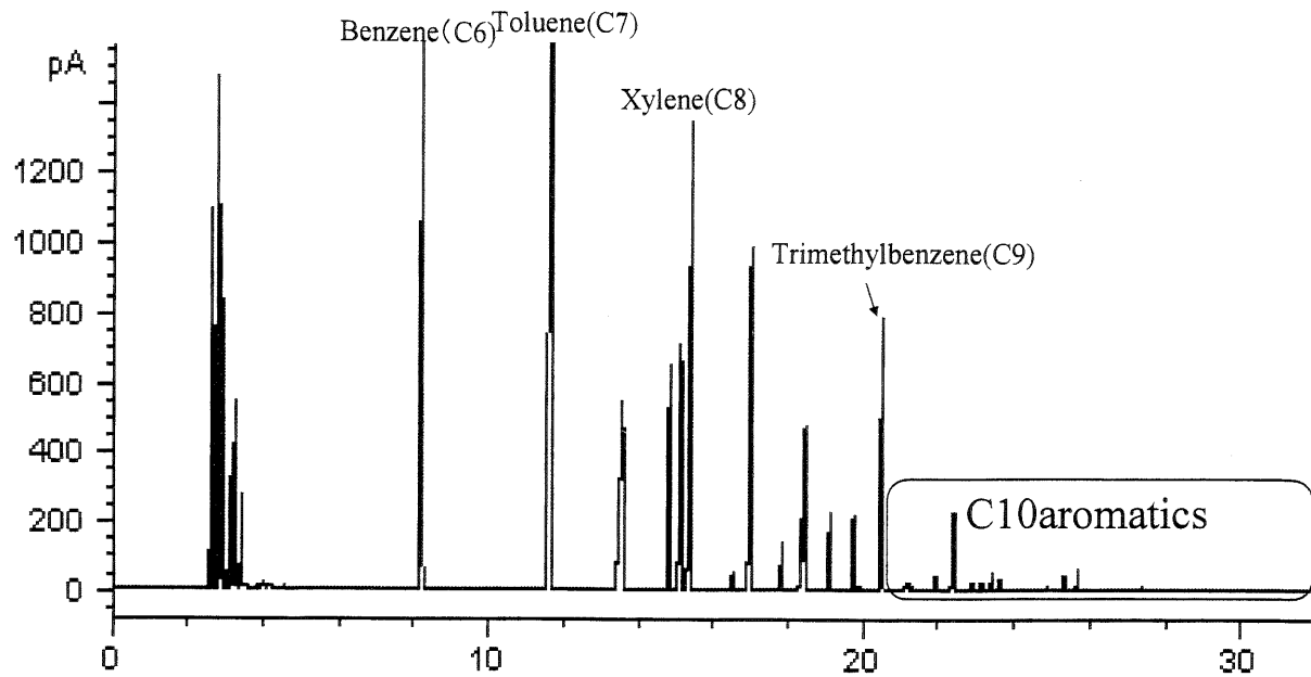
Fig.10 GC chromatogram of Reformate
