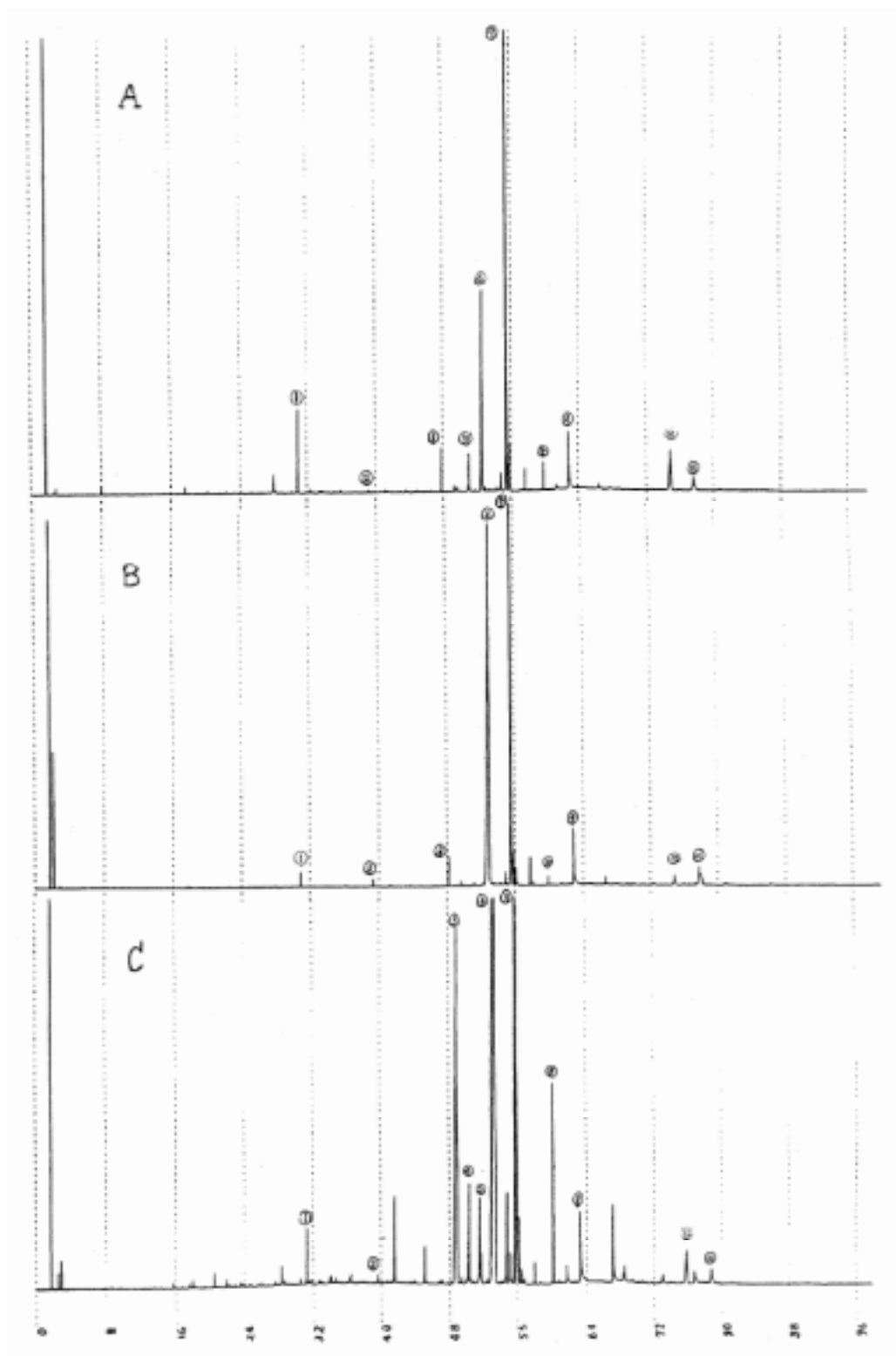
Fig.6 Gas chromatogram of oakmoss absolute oil
