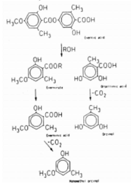
Fig.4 Alcoholysis decomposition of Evernic acid
