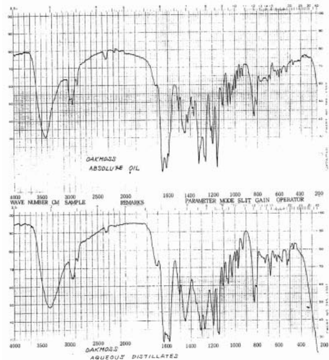
Fig.8 Infrared spectra of oakmoss absolute oil and aqueous distillates
