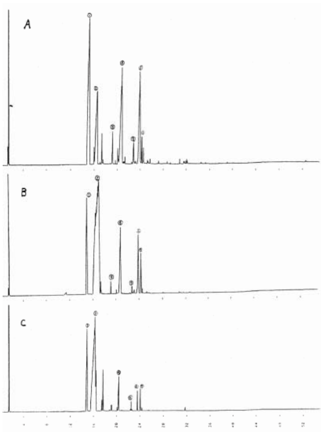
Fig. 7 Gas chromatogram of oakmoss aqueous distillates
