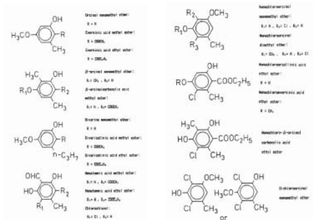
Fig.5 Chemical structures of aromatic compounds produced by depsides decomposition in oakmoss
