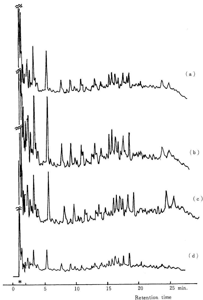
Fig. 2 Pyrograms of Chinese Japan lacquer films at various pyrolytic temperatures
