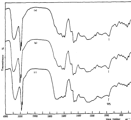
Fig.3 Infrared spectra of cashew lacquer films (curing in room temperature)(カシューNo.53 透) (a) 1 week (b) 3 months (c) 15 months
