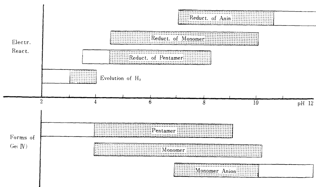
Fig.3 The different forms of Ge and reactions in the phosphate buffer soln. and their dependence on pH.
