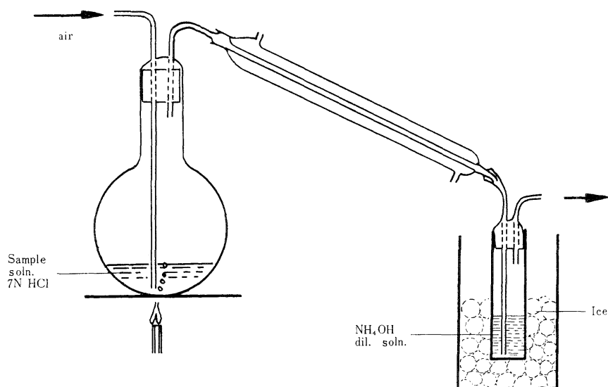
Fig. 1 Apparatus of \text{GeCl}_4 distillation
