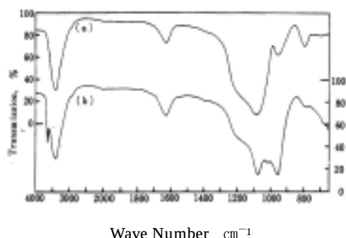
Fig. 9 Infrared Spectra of Acid Treated Chrysotile Asbestos (Sample No.9)
