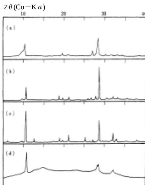
Fig.5 X-Ray diffraction Patterns of Auphybole Group
