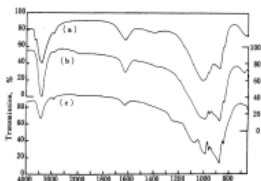
Fig.10 Infrared Spectra of Heat Treated Chrysotile (Sample No.9) (KBr Wafer)
