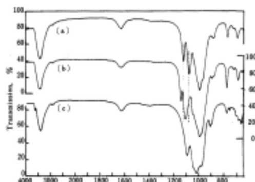
Fig.11 Infrared Spectra of Amphibole Group Asbestos (KBr Wafer)
