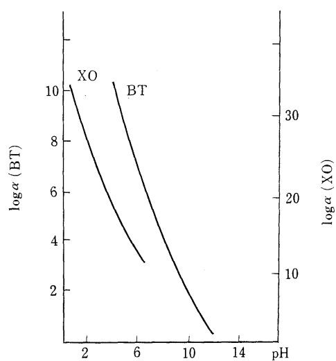
Fig.3 Relationship between \log \alpha I and pH I : BT, XO
