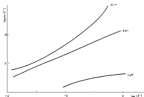
Fig.8 Relationship between \log \alpha_M (F^-) and \log [F^-]
