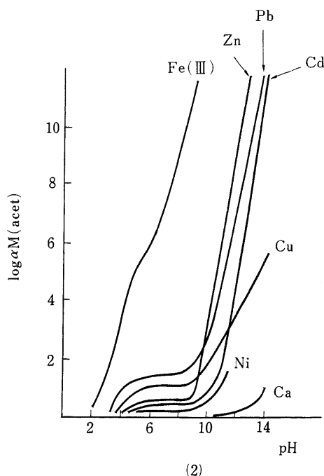
Fig.2 (2) Relationship between \log \alpha M (A) and pH A : acetic acid
