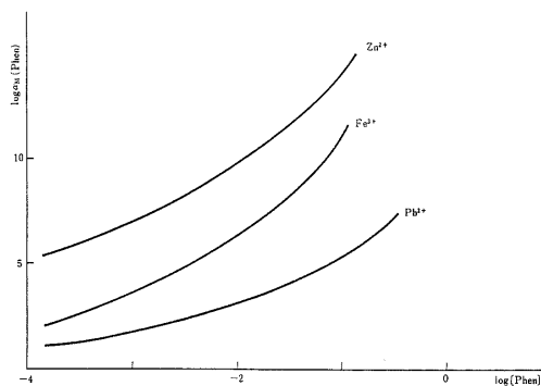
Fig.6 Relationship between \log \alpha_M(Phen) and \log [Phen]
