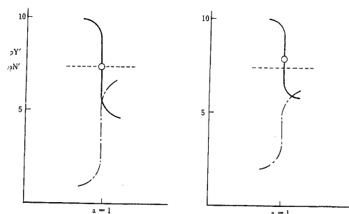
Fig.7 Titration curve after "Phen" added. N : Pb, [Phen]=10^{-2.5}
