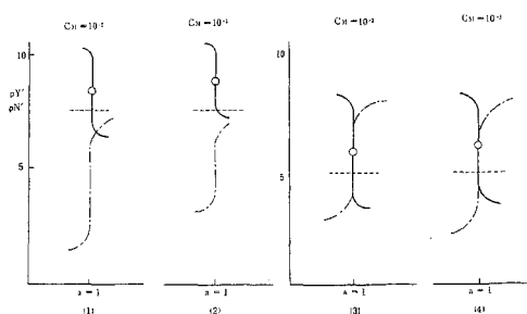
Fig.10 Titration curve after [F^-] added, Effect of the sort of "N"
