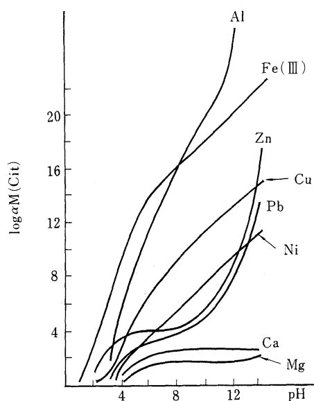
Fig.2 (3) Relationship between \log \alpha M (A) and pH A : citric acid
