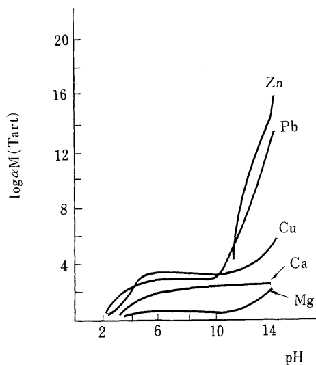
Fig.2 (4) Relationship between \log \alpha M (A) and pH. A : tartaric acid
