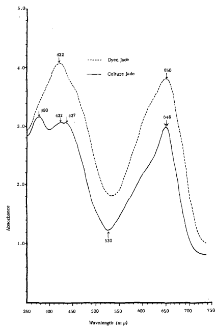
Absorbance Curve of Dyed Jade
