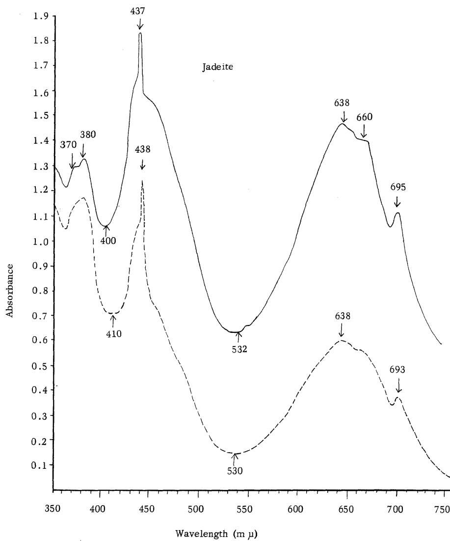
Fig.1. Absorbance Curve of Natural Jadeite
