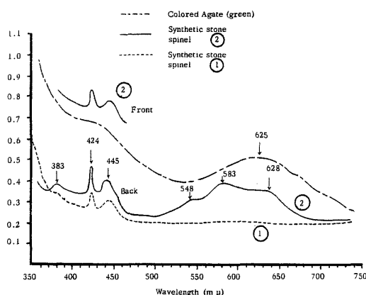
Fig.12. Absorbance Curve of Synthetic Spinel & Colored Agate
