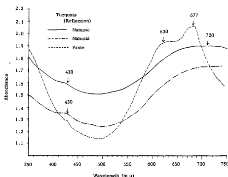
Fig.26. Absorbance Curve of Turquois
