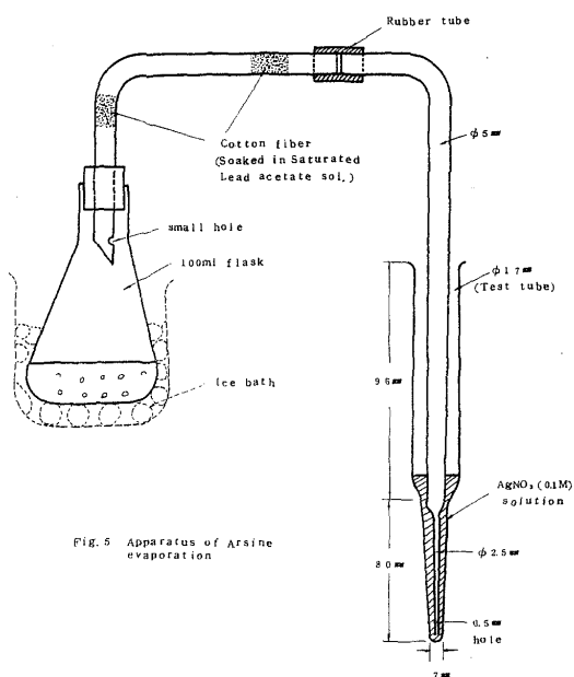
Fig.5 Apparatus of Arsine evaporation
