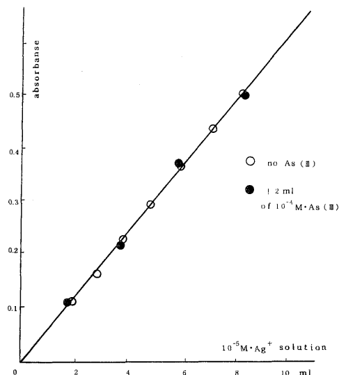
Fig.2 Calibration curve
