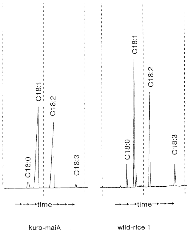
Fig. 4 Gas chromatogram pattern of C18:0~C18:3
