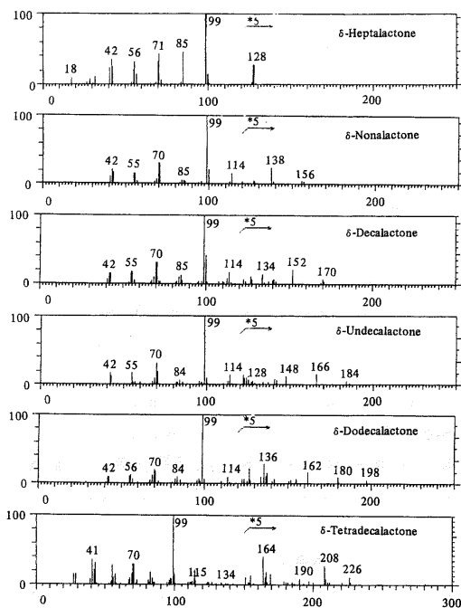
Fig.5 Mass spectra of aroma components (1) \delta -Lactones
