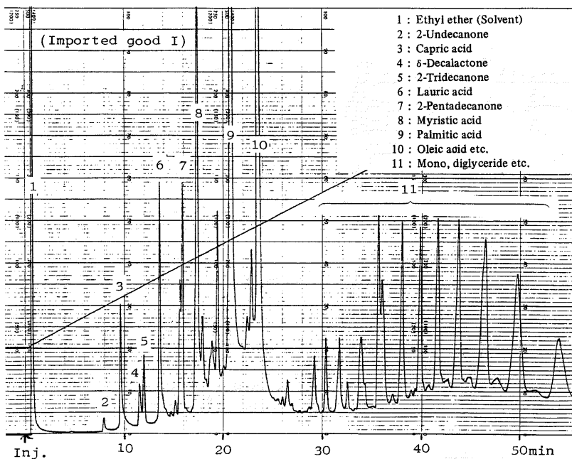
Fig.3 Gas chromatogram of paste type butter flavor(Solution of ethyl ether) GC conditions are cited in paragraph 2・3・2.
