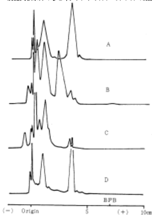
Fig.1 Densitograms of electrophoretogram separated with 9% polyacrylamide gel
