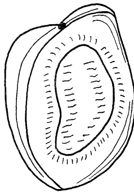
Fig 1. Seed of Tamarindus indica L.( \times 3 )
