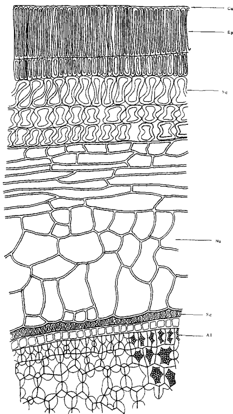
Fig 3. Transvrse section of seed coat and cotyledon (×156)
