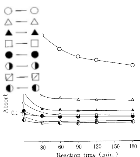
Fig.3 Rate of hydrolysis of phosphate starch synthesized in the laboratory by \beta -amylase
