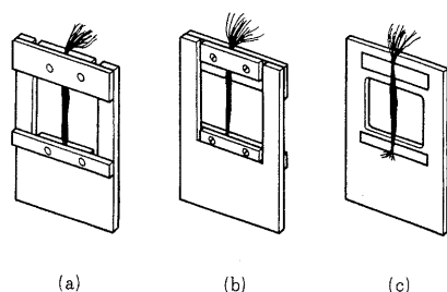
Fig.1 Sample holders for X-ray diffractometry of silk fibroin of our own making ((a) : face, (b) : back) and (c) : by use of adhesive tape
