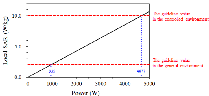
Fig. 5 Comparison between the local SAR over 10 g of arbitrary tissue by 0–5,000 W in the electromagnetic simulation and the guideline value of Radio Radiation Protection Guidelines
