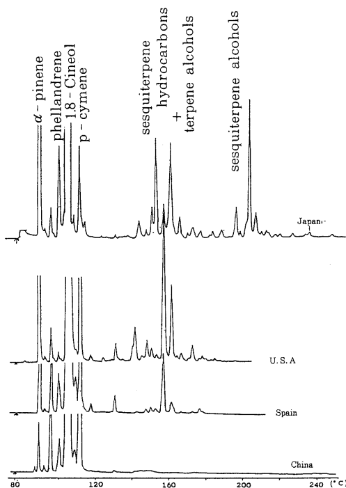
Fig.1 Gaschromatograms of Cineol - Eucalyptus oils
