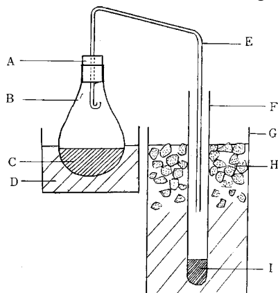
Fig.6 Esterification apparatus
