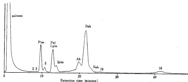
Fig.34 Chromatogram of N-26 resin acid methyl ester Separated rosin acid was stored in dry for 5days at room temperature The GC measurement was carried out immediately after esterification
