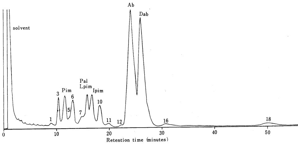
Fig.18 Chromatogram of T-11 tall oil rosin "Acintol R-S"
