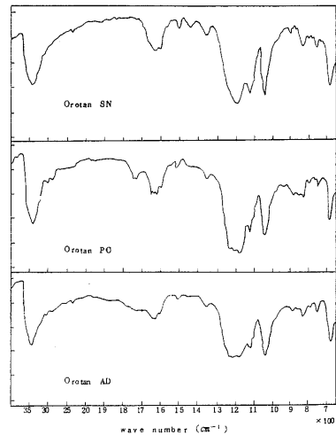
Fig.8. Infrared absorption spectra of naphthalene type syntan. (KBr Wafer)
