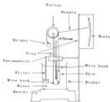
Fig.1 Shrinkage meter
