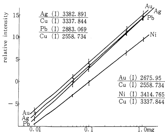
Fig. 6 Calibration curves (Blister copper)
