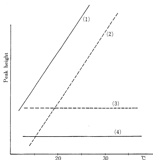
Fig. 7 Effect of temperature to the peak height Supporting electrolyte: 1M \text{HClO}_4 · 0.025M catechol Ge concentration: 34 \mu\text{g}/20\text{ml}
