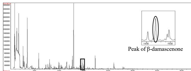
Fig.4 Gas chromatogram of concentrated juice (ii)
