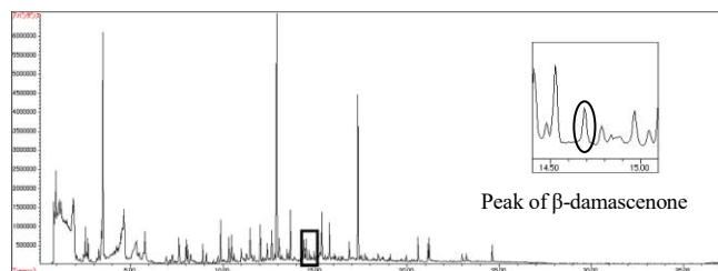
Fig.3 Gas chromatogram of concentrated juice (i)
