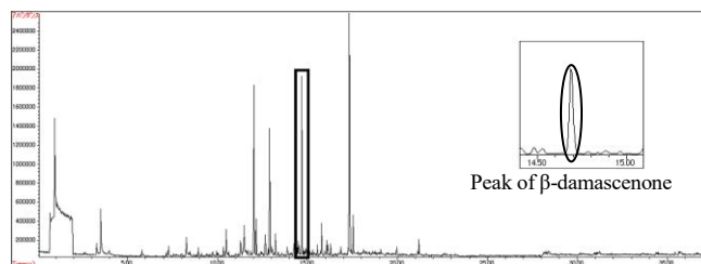
Fig.6 Gas chromatogram of concentrated juice (iv)
