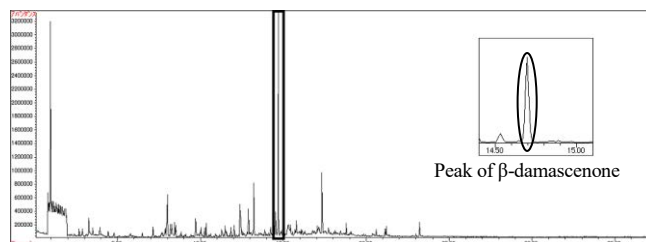
Fig.13 Gas chromatogram of commercially prepared juice from concentrate
