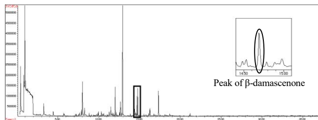
Fig.7 Gas chromatogram of concentrated juice (v)
