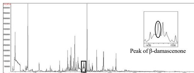
Fig.5 Gas chromatogram of concentrated juice (iii)
