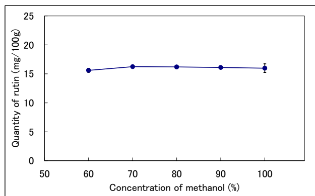
Fig.7 Effect of methanol concentration on the extraction of rutin Rutin was extracted by refluxing in a water bath controlled at 80℃ for 60 min.
