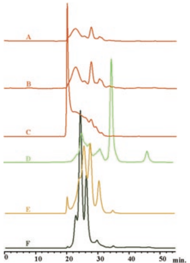
Fig. 14 HPLC chromatograms of honey products (A: a honey added 20% of FGS, B: a honey added 30% of FGS, C: a honey added 40% or below of FGS, D: a honey added oligosaccharides syrup-1, E: a honey added oligosaccharides syrup-2, F: a honey added oligosaccharides syrup-3)
