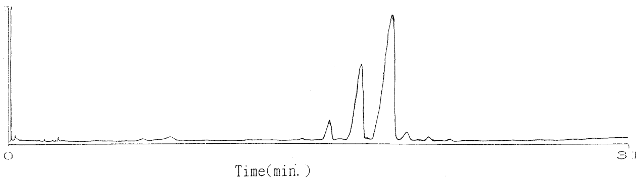
Fig.7 Gas chromatogram of Hydrogenated soy bean oil Column : UltraALLOY-1 (HT) 5m*0.25mm \phi , Film 0.15 \mu m
