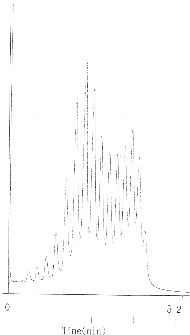
Fig.1 Gas chromatogram of milk fat Colum : Dexil 300 GC 30cm*5mmφ Colum Temp. : 230°C (1min)~360°C (8min) rate 5°C/min Inj./Det. Tem. : 380°C/380°C
