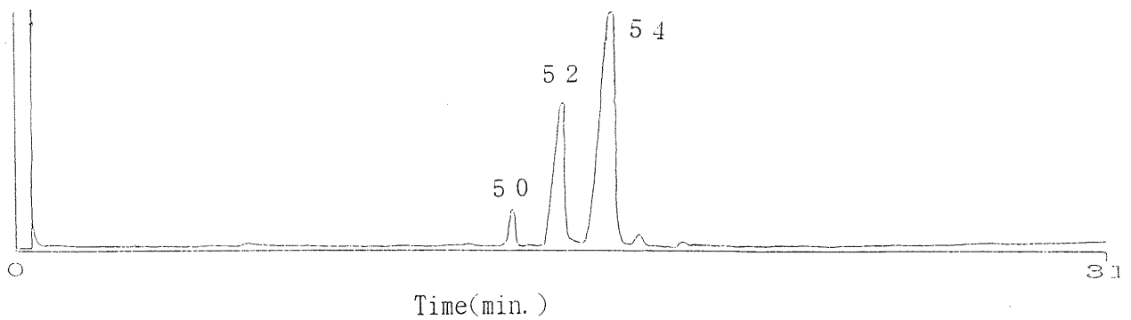
Fig.6 Gas chromatogram of Hydrogenated soy bean oil Column : UltraALLOY-1 (HT) 15m*0.50mm \phi , Film 0.15 \mu m
