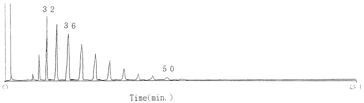
Fig.8 Gas chromatogram of Coconut oil Column : UltraALLOY-1 (HT) 15m*0.50mm \phi , Film 0.15 \mu m
