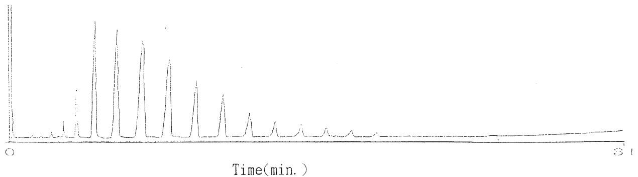
Fig.9 Gas chromatogram of Coconut oil Column : UltraALLOY-1 (HT) 5m*0.25mm \phi , Film 0.15 \mu m
