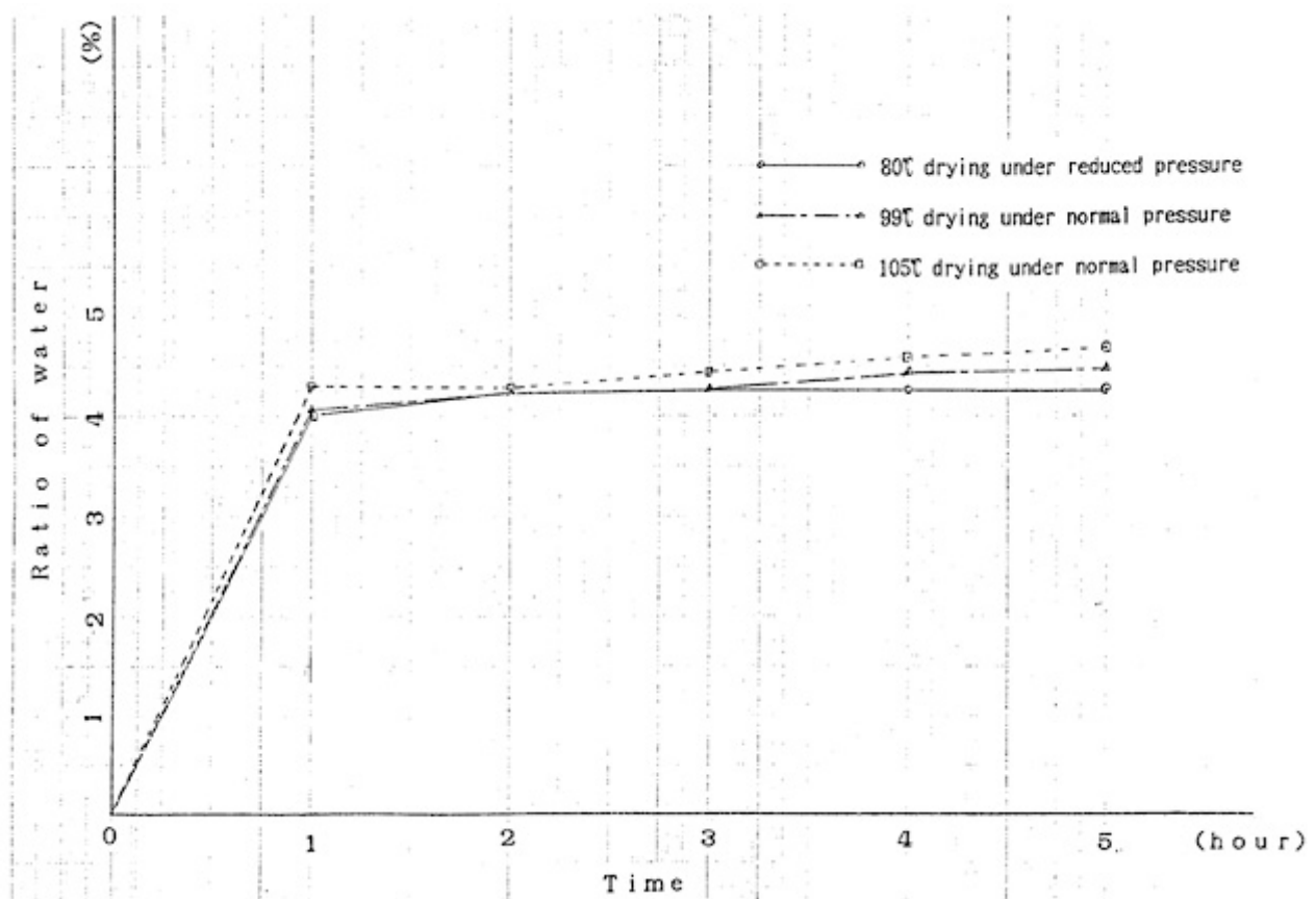
Fig. 1 Relationship between time and ratio of water of skim milk.
