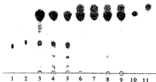
Fig. 2 Thin-layer chromatograms of various vinegars (1)lactose (2)maltose (3)rice vinegar (4)brown rice vinegar (5)job's tears vinegar (6)wine vinegar (7)cider vinegar (8)plum vinegar (9)imported good (10)glucose (11) fructose
