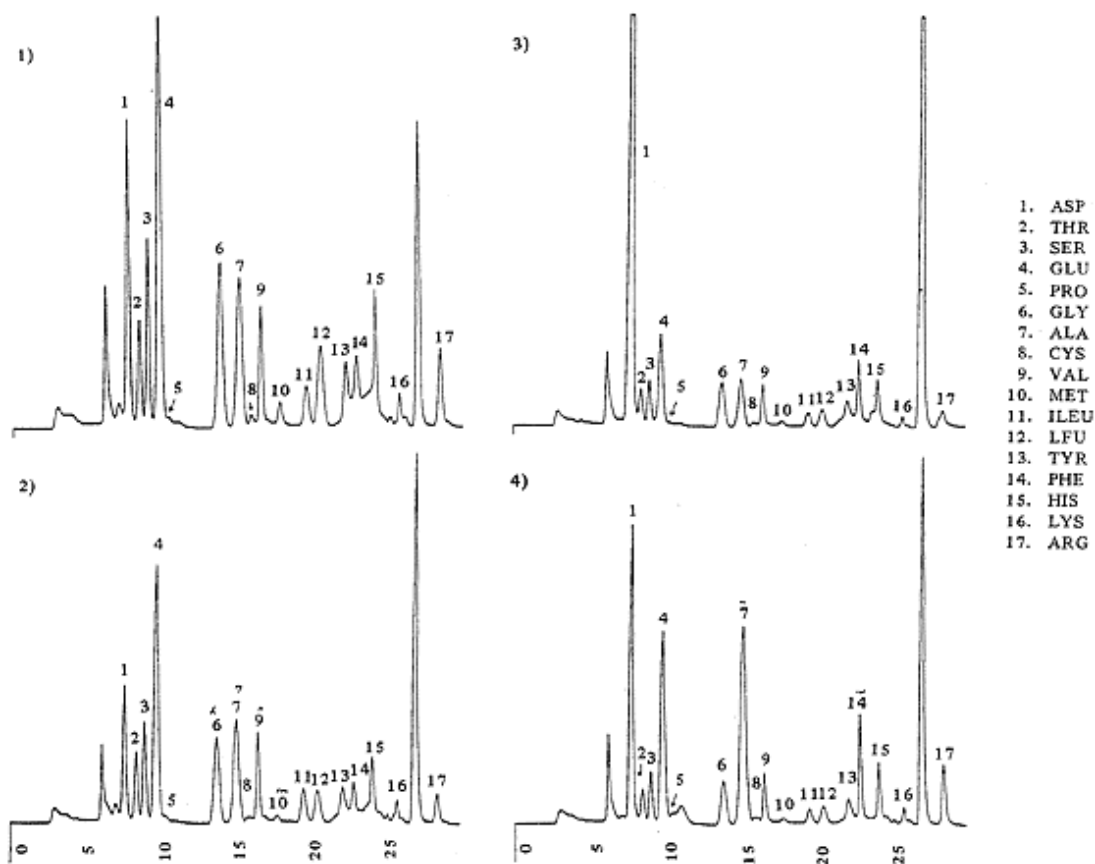
Fig. 3 Total amino acids chromatograms of various vinegars
