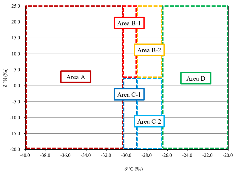
Fig. 2 Carbon-Nitrogen stable isotope ratio plot by the precursor; Area A: Phenylacetone ( \delta^{13}\text{C} : \leq -30.4 ‰), Area B-1: Mixture of Ephedrines (extracted from Ephedra ) and Phenylacetone ( \delta^{13}\text{C} : > -30.4 ‰ and \leq -29.2 ‰, \delta^{15}\text{N} : > 2.5 ‰), Area B-2: Ephedrines extracted from Ephedra ( \delta^{13}\text{C} : > -29.2 ‰ and \leq -26.5 ‰, \delta^{15}\text{N} : > 2.5 ‰), Area C-1: Mixture of Ephedrines (synthesized from chemicals) and Phenylacetone ( \delta^{13}\text{C} : > -30.4 ‰ and \leq -29.2 ‰, \delta^{15}\text{N} : \leq 2.5 ‰), Area C-2: Ephedrines synthesized from chemicals ( \delta^{13}\text{C} : > -29.2 ‰ and \leq -26.5 ‰, \delta^{15}\text{N} : \leq 2.5 ‰) and Area D: Ephedrines generated from fermented sugar ( \delta^{13}\text{C} : > -26.5 ‰)
