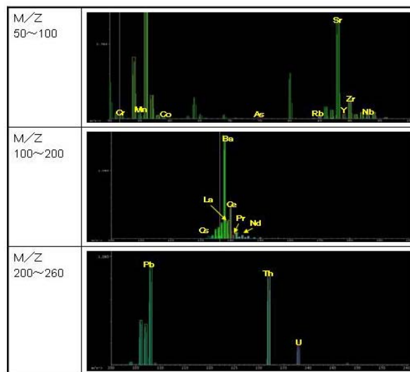
Fig. 1 Mass spectra of anthracite by ICP-MS
