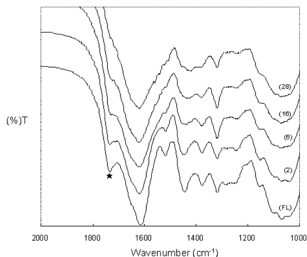
Fig.4 Infrared spectra of our own leaf moulds and fallen leaf. (28), (16), (6), and (2) are our own leaf moulds, each number in parentheses expresses decay time (week). (FL) is fallen leaf. ★ represents peak of 1740\text{ cm}^{-1} .
