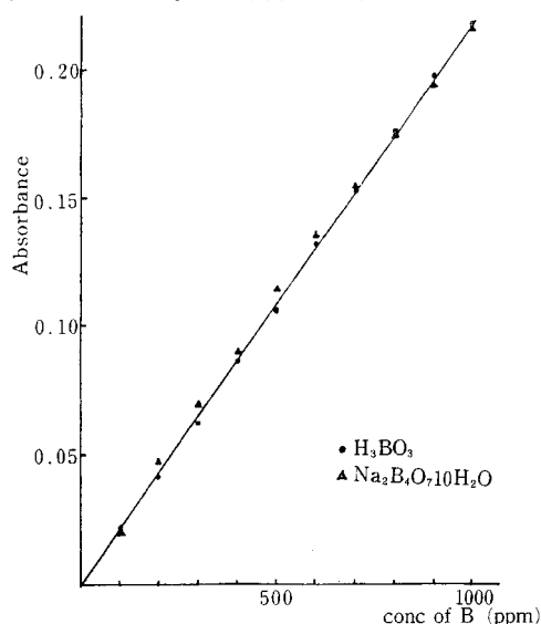
Fig. 11 Calibration curve of boron atomic absorption
